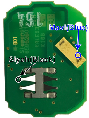
"ZFH-C07 / ZFH-C07-02 CABLE" (ALT / BOTTOM)
