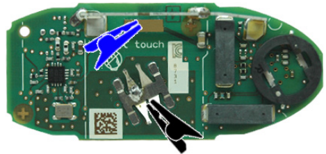
"ZFH-C12 CABLE" (ALT/ BOTTOM)
