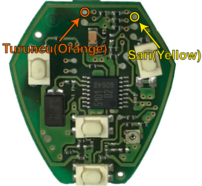
"ZFH-C07 / ZFH-C07-02 CABLE" (ÜST / TOP)
