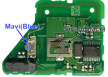
"ZFH-C07 / ZFH-C07-02 CABLE" (ALT / BOTTOM)
