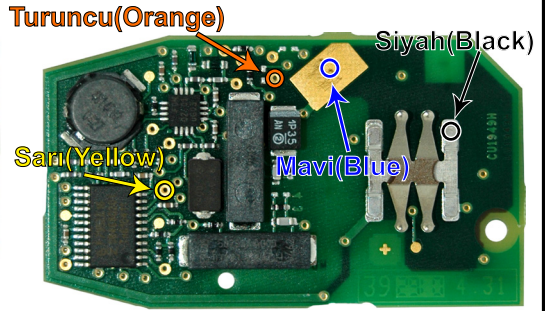
"ZFH-C07 / ZFH-C07-02 CABLE" (ALT / BOTTOM)
