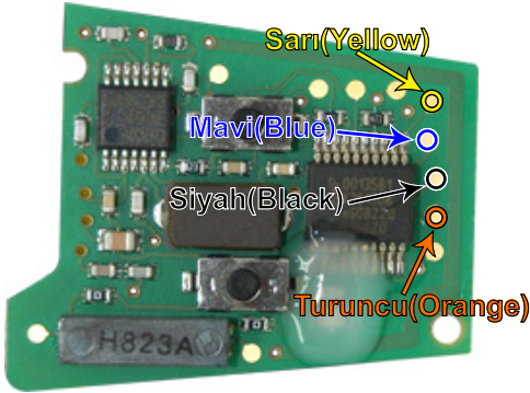
"ZFH-C07 / ZFH-C07-02 CABLE" (ÜST / TOP)
