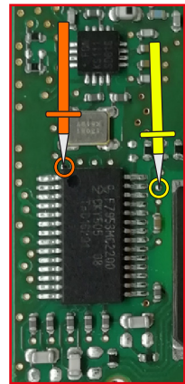
"ZFH-C12 CABLE " (ALT / BOTTOM)
