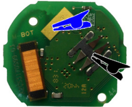
"ZFH-C12 CABLE " (ALT/ BOTTOM)
