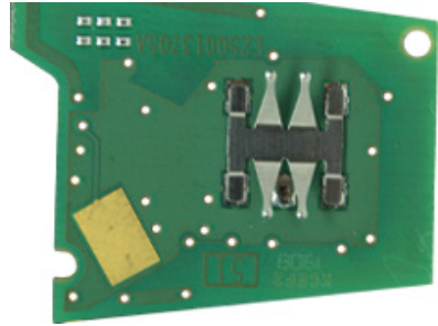
"ZFH-C07 / ZFH-C07-02 CABLE" (ALT / BOTTOM)
