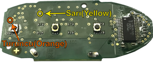
"ZFH-C07 / ZFH-C07-02 CABLE" (ÜST / TOP)
