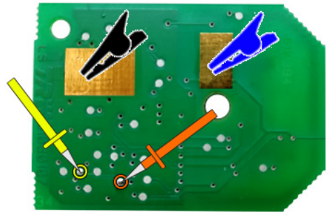
"ZFH-C12 CABLE " (ALT/ BOTTOM)
