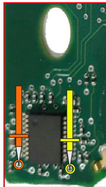
"ZFH-C12 CABLE " (ÜST / TOP)
