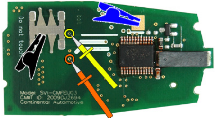
"ZFH-C12 CABLE" (ALT/ BOTTOM)
