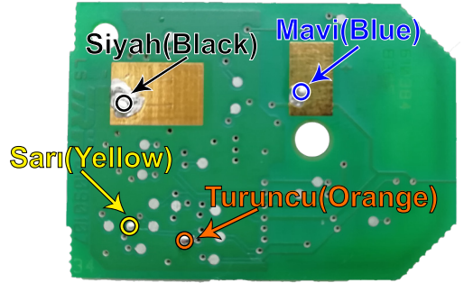
"ZFH-C07 / ZFH-C07-02 CABLE" (ALT / BOTTOM)
