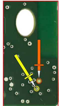
"ZFH-C12 CABLE " (ALT / BOTTOM)
