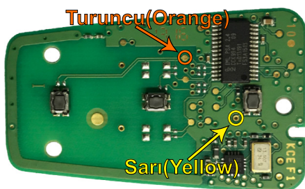
"ZFH-C07 / ZFH-C07-02 CABLE" (ÜST / TOP)
