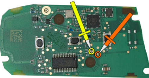
"ZFH-C12 CABLE " (ÜST/ TOP)
