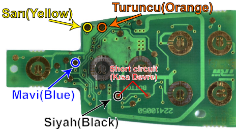
"ZFH-C07 / ZFH-C07-02 CABLE" (ÜST / TOP)
