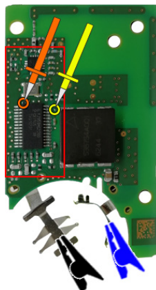
"ZFH-C12 CABLE " ALT / BOTTOM)
