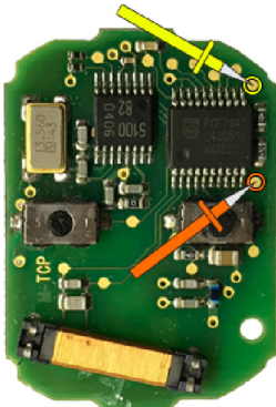
"ZFH-C12 CABLE " (ÜST/ TOP)
