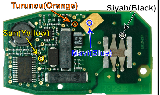
"ZFH-C07 / ZFH-C07-02 CABLE" (ALT / BOTTOM)
