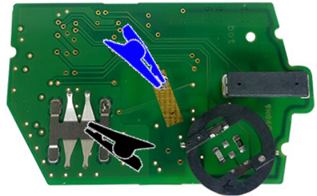
"ZFH-C12 CABLE " (ALT/ BOTTOM)
