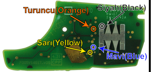
"ZFH-C07 / ZFH-C07-02 CABLE" (ALT / BOTTOM)
