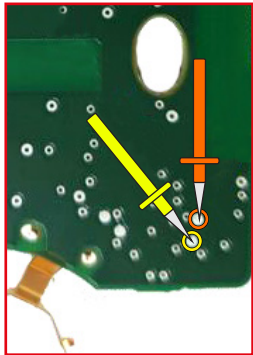
"ZFH-C12 CABLE" (ALT / BOTTOM)
