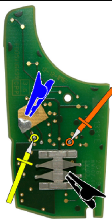
"ZFH-C12 CABLE" (ALT / BOTTOM)
