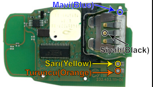
"ZFH-C07 / ZFH-C07-02 CABLE" (ALT / BOTTOM)
