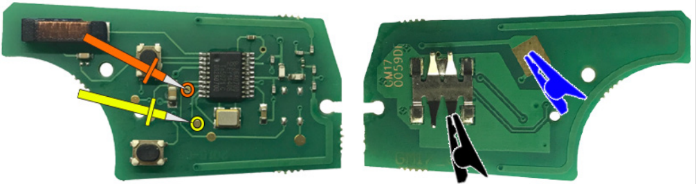
"ZFH-C12 CABLE " (ALT/ BOTTOM)
