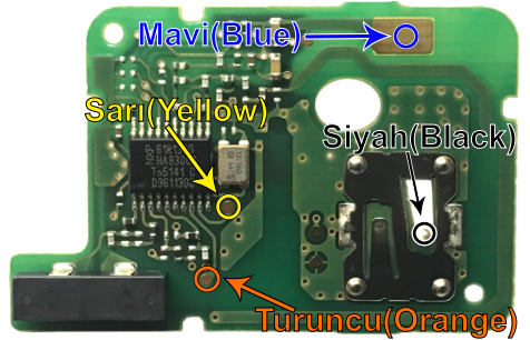
"ZFH-C07 / ZFH-C07-02 CABLE" (ALT / BOTTOM)
