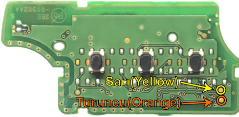
"ZFH-C07 / ZFH-C07-02 CABLE" (ÜST / TOP)
