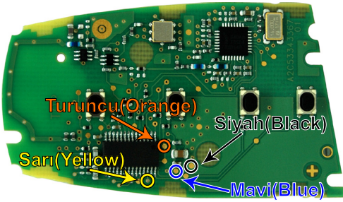
"ZFH-C07 / ZFH-C07-02 CABLE" (ÜST / TOP)
