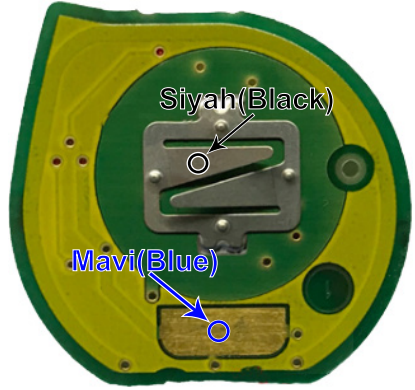
"ZFH-C07 / ZFH-C07-02 CABLE" ALT / BOTTOM)
