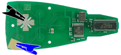
"ZFH-C12 CABLE" (ALT/ BOTTOM)
