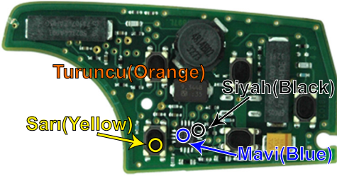
"ZFH-C07 / ZFH-C07-02 CABLE" (ÜST / TOP)
