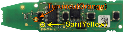
"ZFH-C07 / ZFH-C07-02 CABLE" (ÜST / TOP)
