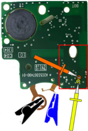
"ZFH-C12 CABLE" (ALT / BOTTOM)
