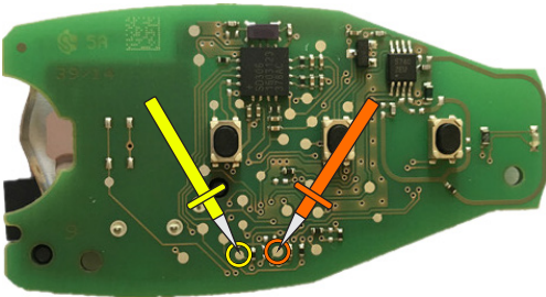
"ZFH-C12 CABLE " (ÜST / TOP)
