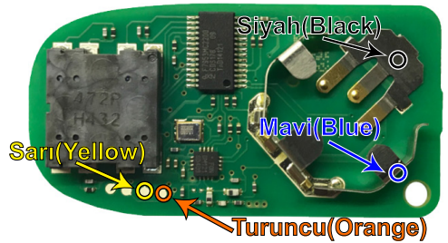
"ZFH-C07 / ZFH-C07-02 CABLE" (ALT / BOTTOM)
