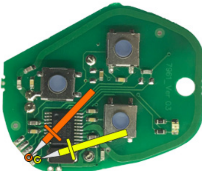
"ZFH-C12 CABLE" (ÜST/ TOP)
