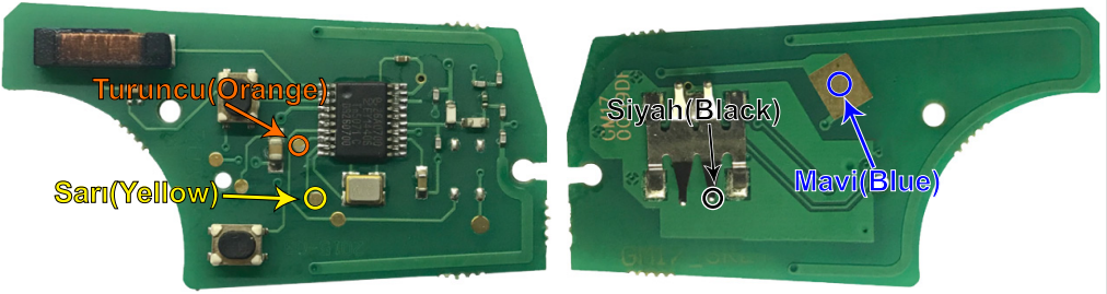
"ZFH-C07 / ZFH-C07-02 CABLE" (ÜST / TOP)
