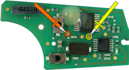
"ZFH-C12 CABLE" (ÜST/ TOP)
