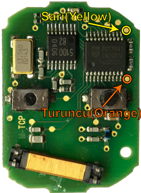
"ZFH-C07 / ZFH-C07-02 CABLE" (ÜST / TOP)
