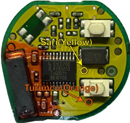
"ZFH-C07 / ZFH-C07-02 CABLE" (ÜST / TOP)
