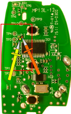
"ZFHC12 CABLE" (ÜST/ TOP)
