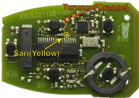
"ZFH-C07 / ZFH-C07-02 CABLE" (ÜST / TOP)
