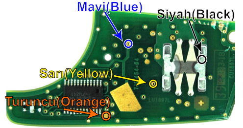
"ZFH-C07 / ZFH-C07-02 CABLE" (ALT / BOTTOM)
