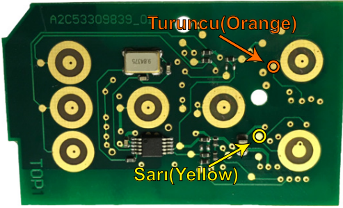
"ZFH-C07 / ZFH-C07-02 CABLE" (ÜST / TOP)
