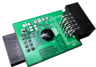
PCF79XX Remote Recycling Adapter
