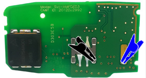
"ZFH-C12 CABLE " (ALT/ BOTTOM)
