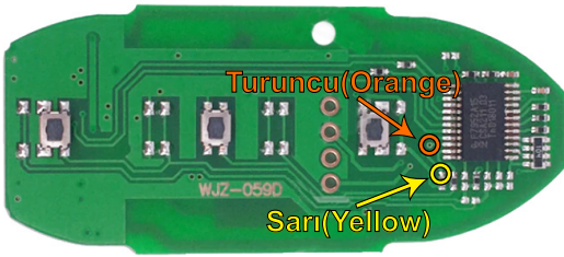
"ZFH-C07 / ZFH-C07-02 CABLE" (ÜST / TOP)
