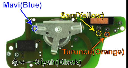
"ZFH-C07 / ZFH-C07-02 CABLE" (ALT / BOTTOM)
