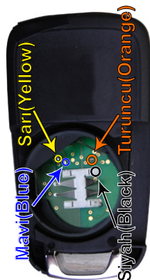
"ZFH-C07 / ZFH-C07-02 CABLE" (ALT / BOTTOM)
