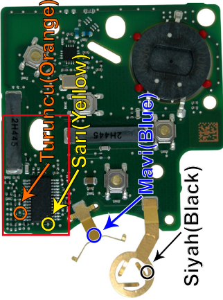
"ZFH-C07 / ZFH-C07-02 CABLE" (ÜST / TOP)
