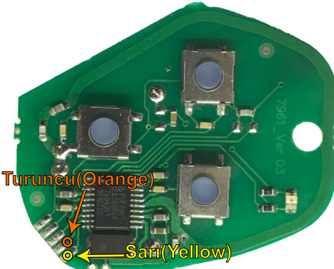
"ZFH-C07 / ZFH-C07-02 CABLE" (ÜST / TOP)
