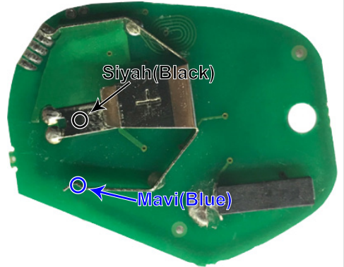
"ZFH-C07 / ZFH-C07-02 CABLE" (ALT / BOTTOM)
