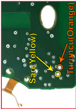
"ZFH-C07 / ZFH-C07-02 CABLE" (ALT / BOTTOM)
