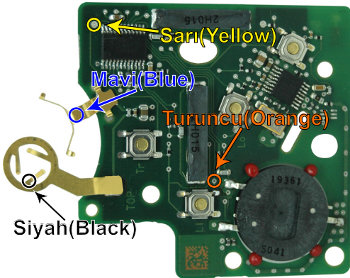
"ZFH-C07 / ZFH-C07-02 CABLE" (ÜST / TOP)
