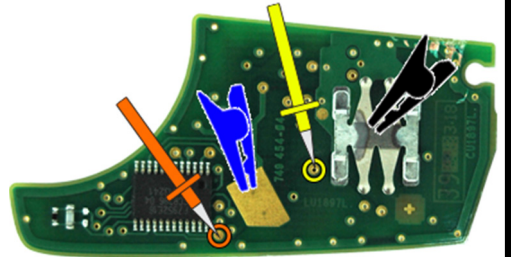
"ZFH-C12 CABLE " (ALT/ BOTTOM)
