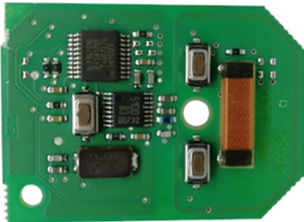
"ZFH-C12 CABLE " (ÜST/ TOP)
