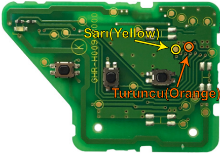
"ZFH-C07 / ZFH-C07-02 CABLE" (ÜST / TOP)
