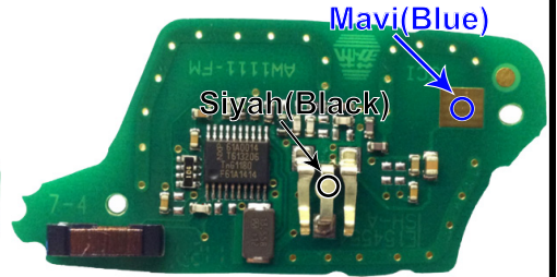
"ZFH-C07 / ZFH-C07-02 CABLE" (ALT / BOTTOM)
