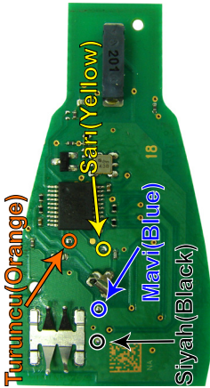
"ZFH-C07 / ZFH-C07-02 CABLE" (ALT / BOTTOM)
