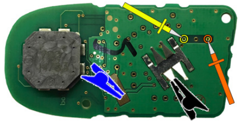
"ZFH-C12 CABLE" (ALT/ BOTTOM)
