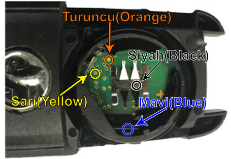
"ZFH-C07 / ZFH-C07-02 CABLE" (ALT / BOTTOM)
