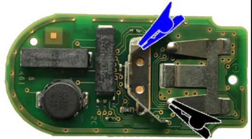
"ZFH-C12 CABLE " (ALT/ BOTTOM)
