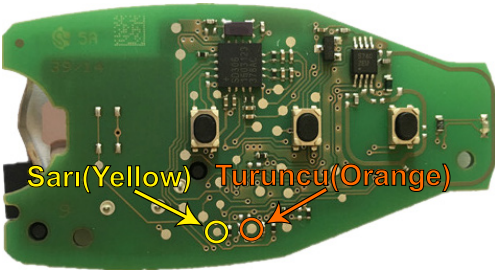
"ZFH-C07 / ZFH-C07-02 CABLE" (ÜST / TOP)
