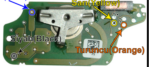
"ZFH-C07 / ZFH-C07-02 CABLE" (ALT / BOTTOM)
