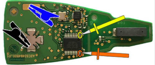
"ZFH-C12 CABLE" (ALT/ BOTTOM)
