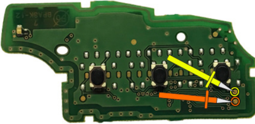
"ZFH-C12 CABLE" (ÜST/ TOP)
