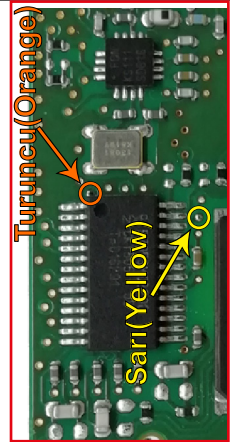
"ZFH-C07 / ZFH-C07-02 CABLE" (ALT / BOTTOM)
