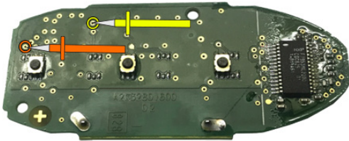
"ZFH-C12 CABLE" (ÜST/ TOP)
