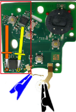
"ZFH-C12 CABLE " (ÜST / TOP)
