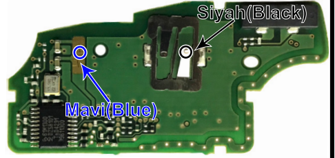
"ZFH-C07 / ZFH-C07-02 CABLE" (ALT / BOTTOM)
