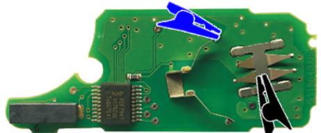
"ZFH-C12 CABLE " (ALT/ BOTTOM)
