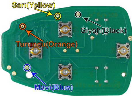
"ZFH-C07 / ZFH-C07-02 CABLE" (ÜST / TOP)
