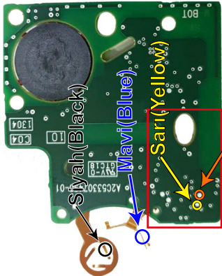
Turuncu (Orange) "ZFH-C07 / ZFH-C07-02 CABLE" (ALT / BOTTOM)
