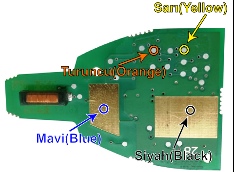
"ZFH-C07 / ZFH-C07-02 CABLE" (ALT / BOTTOM)
