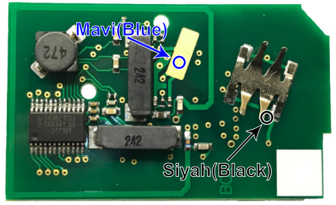
"ZFH-C07 / ZFH-C07-02 CABLE" (ALT / BOTTOM)
