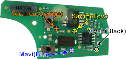
"ZFH-C07 / ZFH-C07-02 CABLE" (ÜST / TOP)
