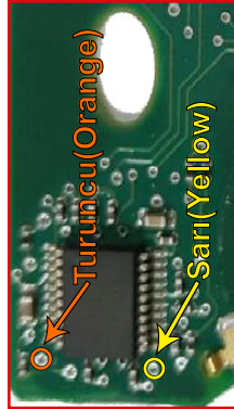
"ZFH-C07 / ZFH-C07-02 CABLE" (ÜST / TOP)
