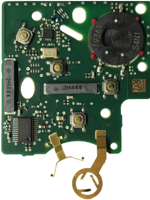
"ZFH-C07 / ZFH-C07-02 CABLE" (ÜST / TOP)
