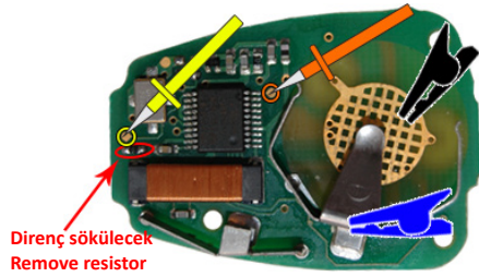
"ZFH-C12 CABLE" (ALT / BOTTOM)
