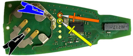
"ZFH-C12 CABLE" (ALT/ BOTTOM)
