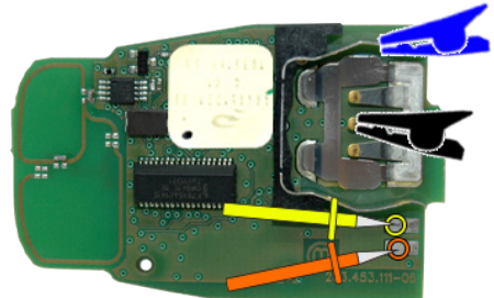
"ZFH-C12 CABLE" (ALT/ BOTTOM)
