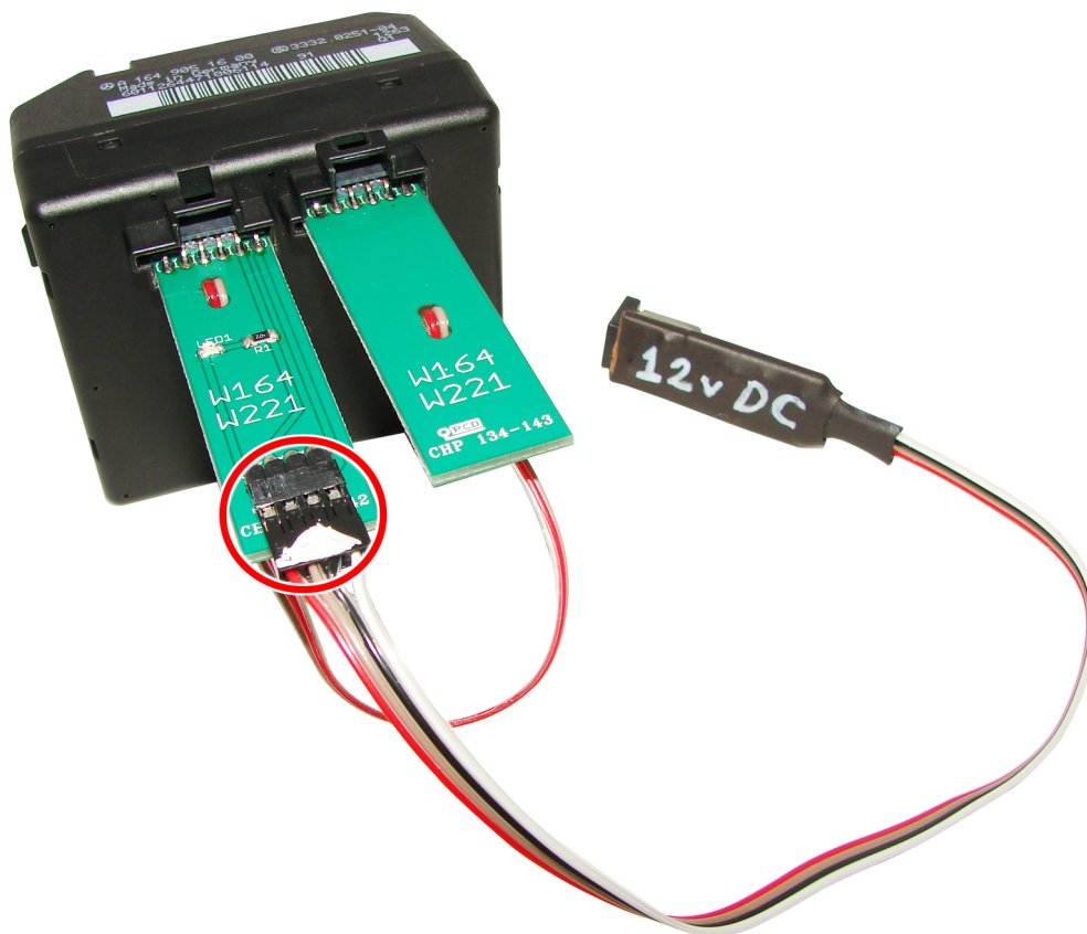
Test Kit
